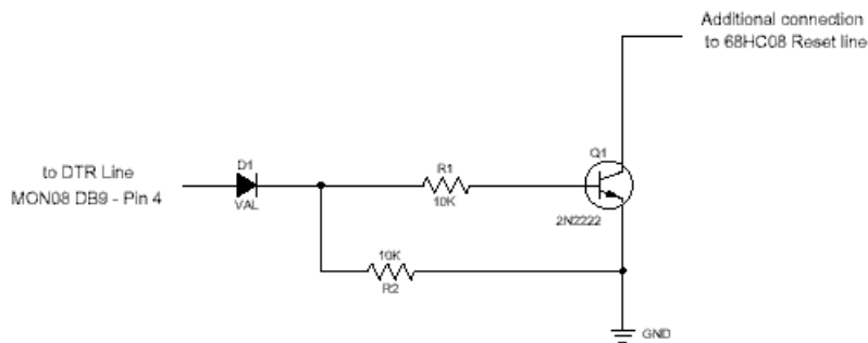
Figure 6-16: Additional Connection To Reset From DB9
