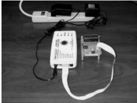
Figure 2-7: Via Power In Jack and Pin 15 of Cyclone
