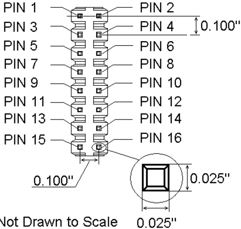
Figure 2-2: 16-Pin Header Mechanical Drawing
