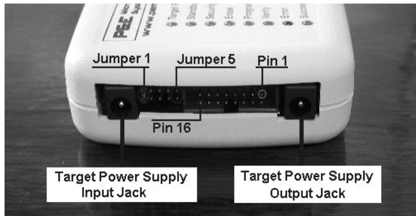
Figure 2-1: Power Connector Locations
