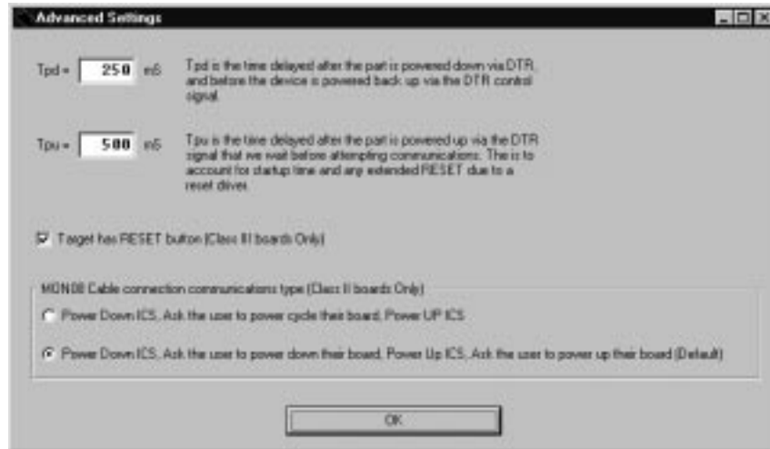
Figure 6-23: Target Hardware Type: Advanced Settings Dialog
