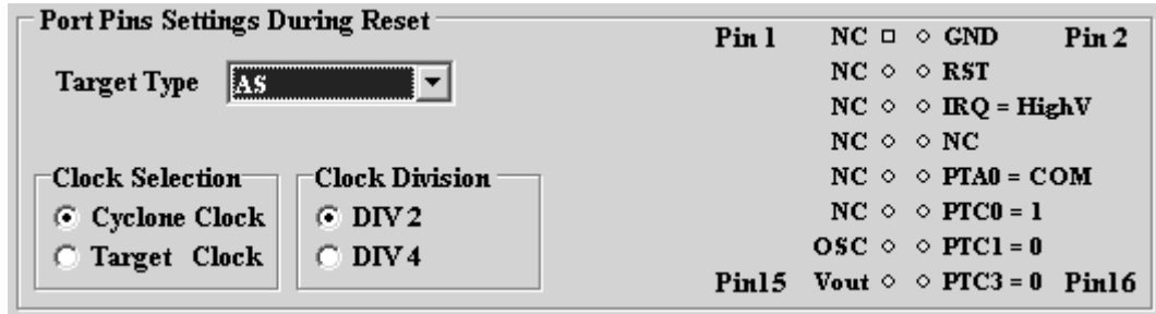
Figure 3-3: 68HC908AS Family MON08 Pinout
