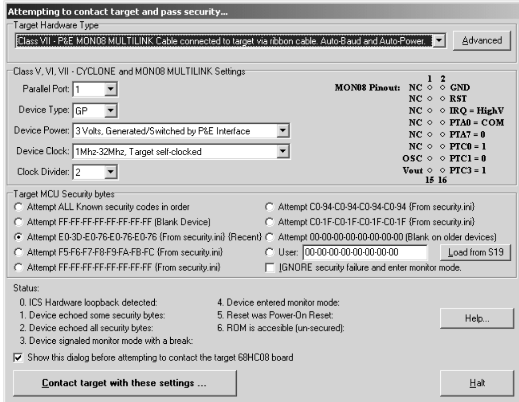
Figure 6-19: Class V, VI, VII Target And Security Dialog
