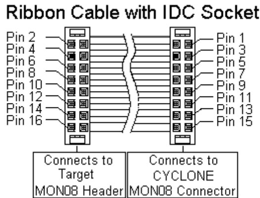
Figure 2-4: Ribbon Cable Diagram
