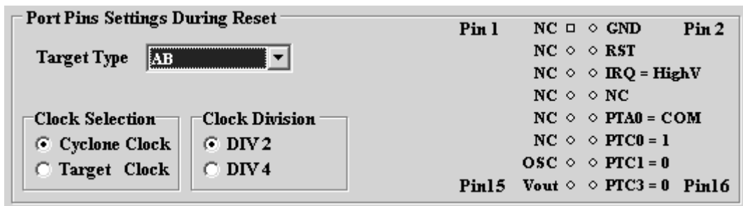
Figure 5-2: Port Pin Settings - 68HC908AB Family
