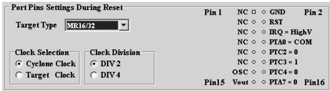
Figure 3-21: 68HC908MR16/32 Family MON08 Pinout
