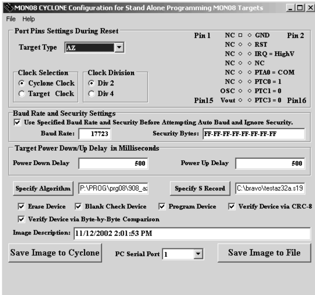
Figure 5-1: Configuration Dialog
