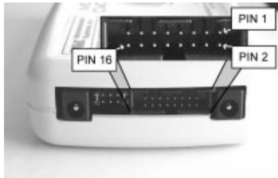
Figure 2-3: MON08 Connector Pin Location
